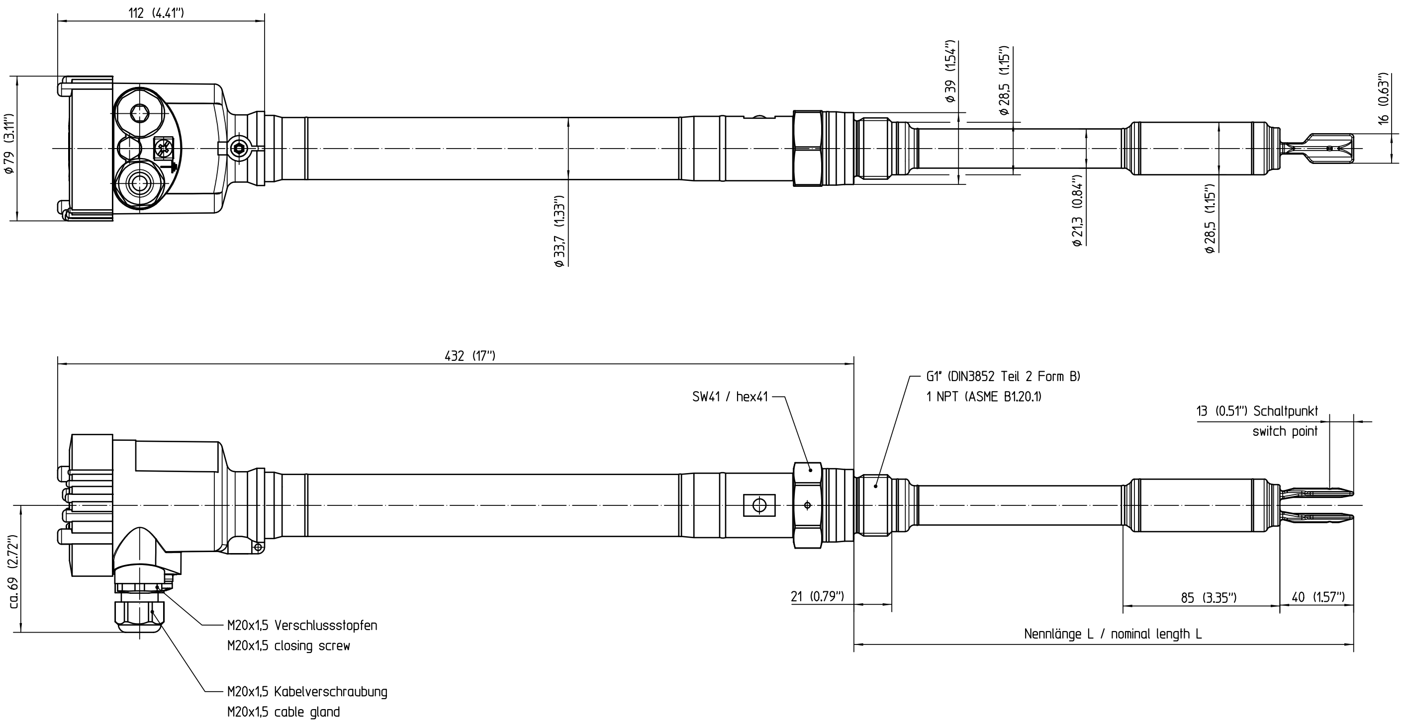
Bemassungen / Dimensions: mm (inches)
